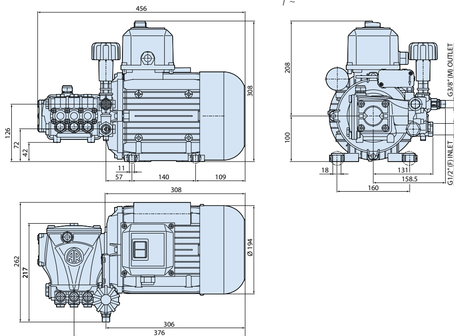
GR. 100 motor hollow shaft
